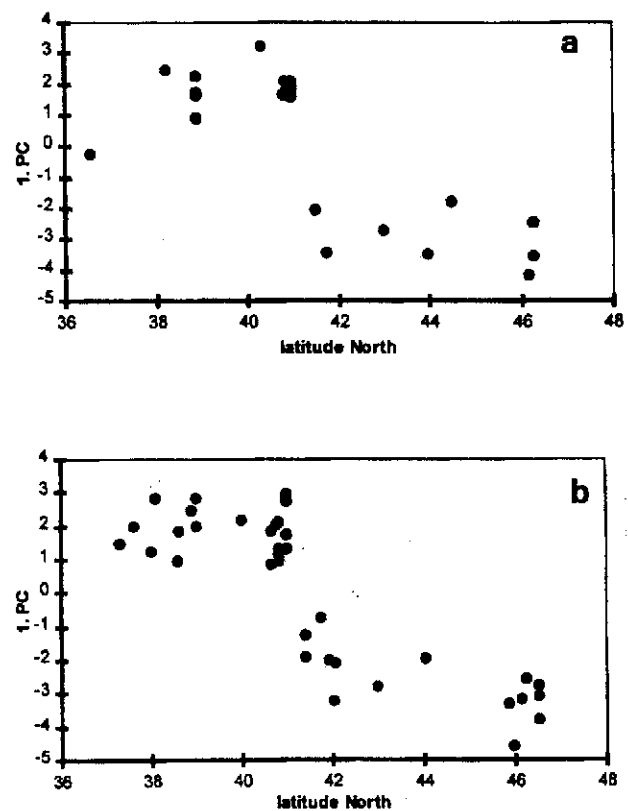
FIG. 4. Scatter diagram of the 1st. PC scores of PCA 3 of females (a) and males (b) on a transect running along the Apennine Peninsula. Sardinia excluded.
